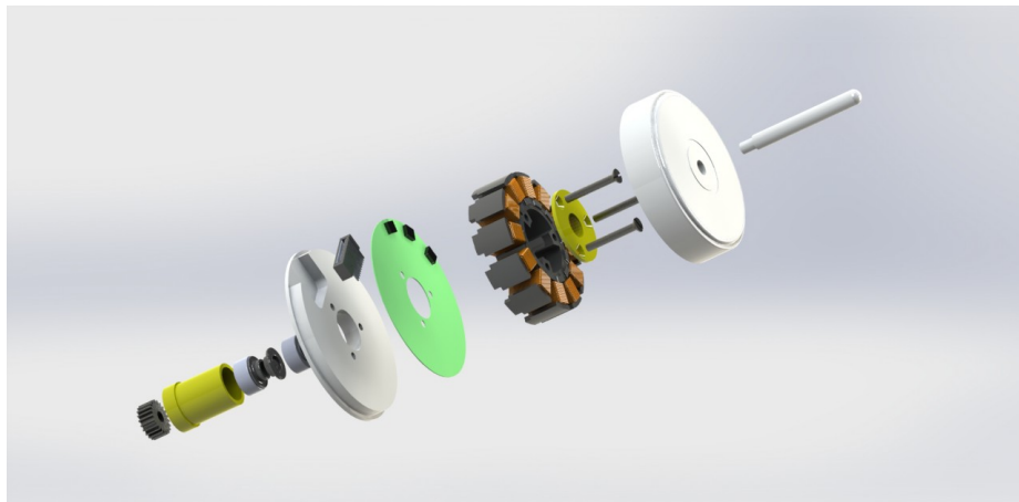
Fig. 7. Parsian modified Maxon EC45 motor disassembled .
