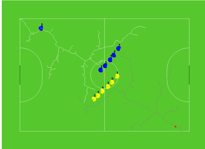
Fig. 15. Try finding path with RRT from 2 ways. Robot toward the destination (white) and Destination toward robot (gray)
