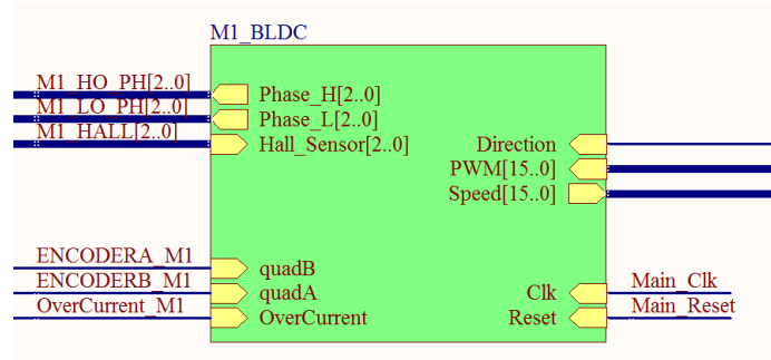
Fig. 12. BLDC Motor controller block.
