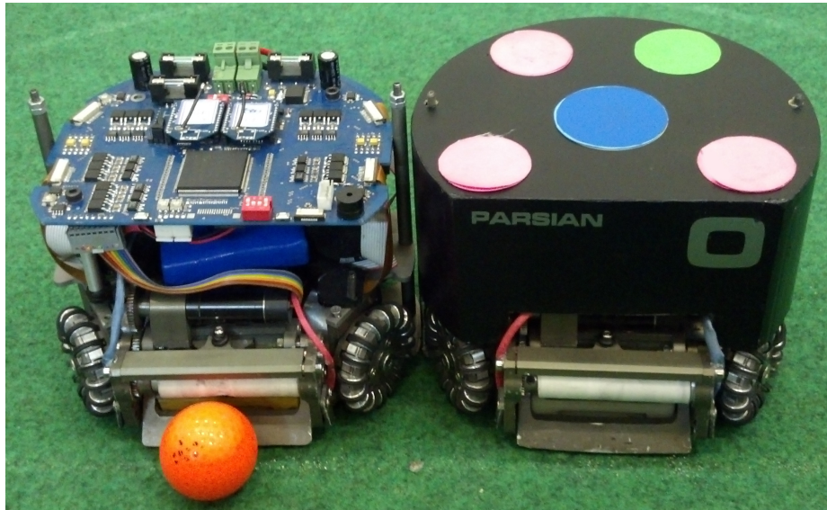
Fig. 2. Our current robots with and without cover
