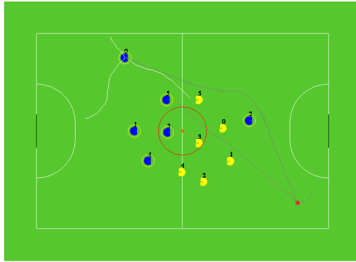
Fig. 17. Smooth path generated from RRT considering the angle between new extension and last branch.
