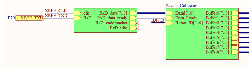
Fig. 11. Receiver and packet selector Verilog blocks.
