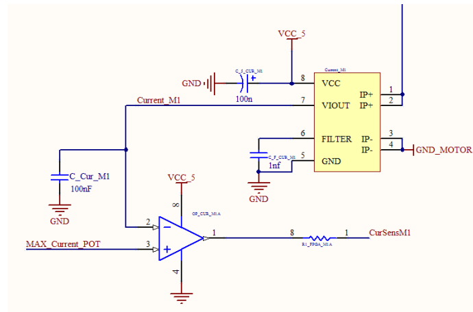
Fig. 13. Overcurrent protection circuit.
