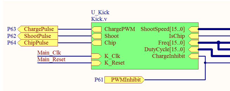
Fig. 14. Kicker Verilog block.
