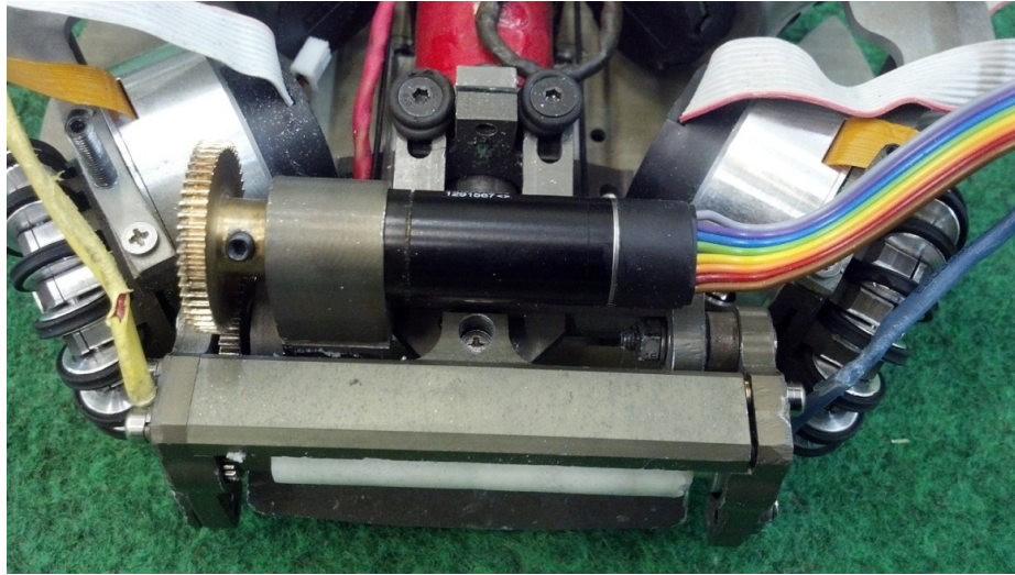
Fig. 9. Robots adjustable 2DOF suspension system
