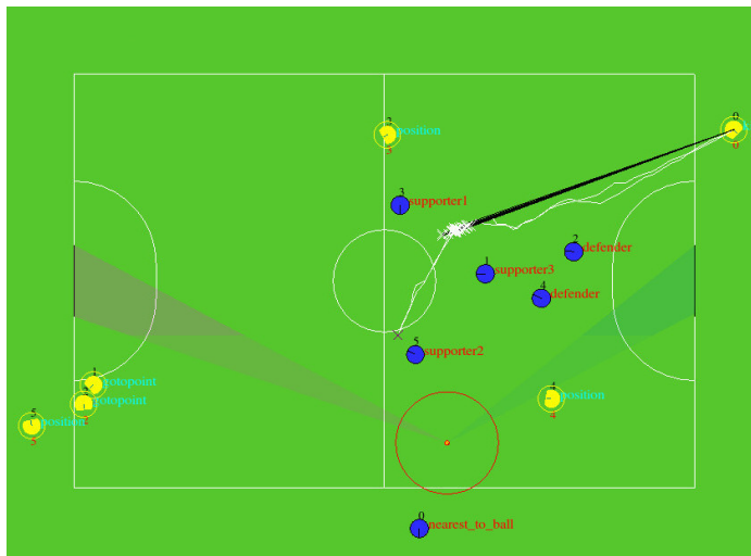
Fig. 16. The RRT result for robot shown by white and the black segment shows how we extract an straight line from that.
