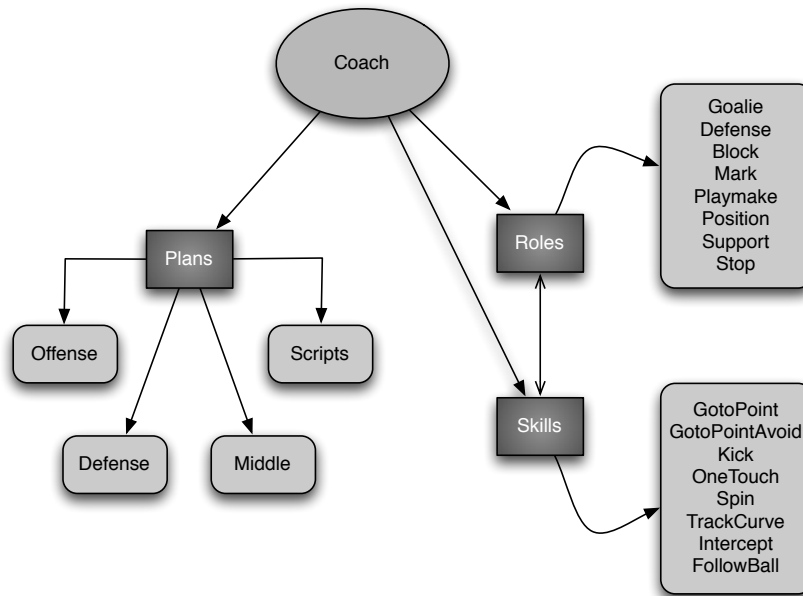
Fig. 19. The hierarchy of coach stucture
