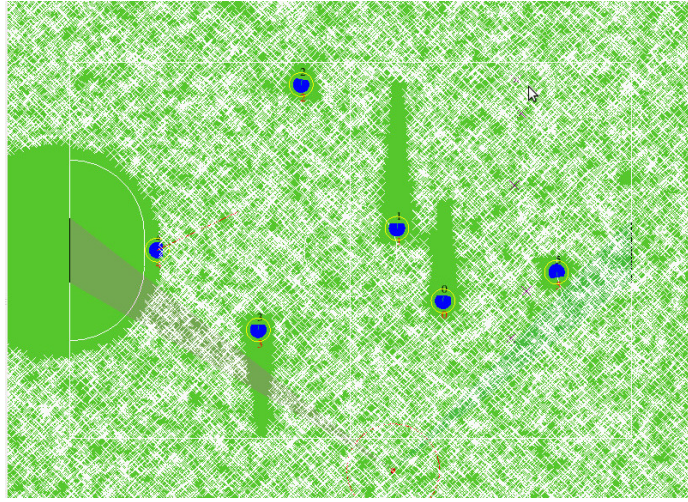
Fig. 18. Moving obstacles and how we consider their speed to avoid collision, the white crosses are possible random states which is safe to go.
