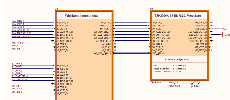
Fig. 10. TSK3000 soft processor connected to blocks via Wishbone Interconnect.
