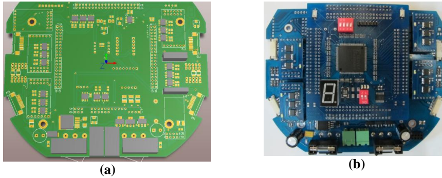
Fig. 5. (a) 3D design (b) real hardware
