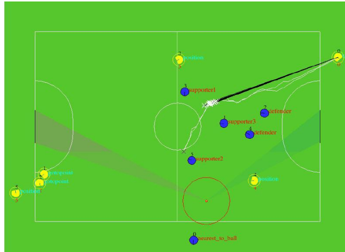
Fig. 18. The RRT result for robot shown by white and the black segment shows how we extract an straight line from that.
