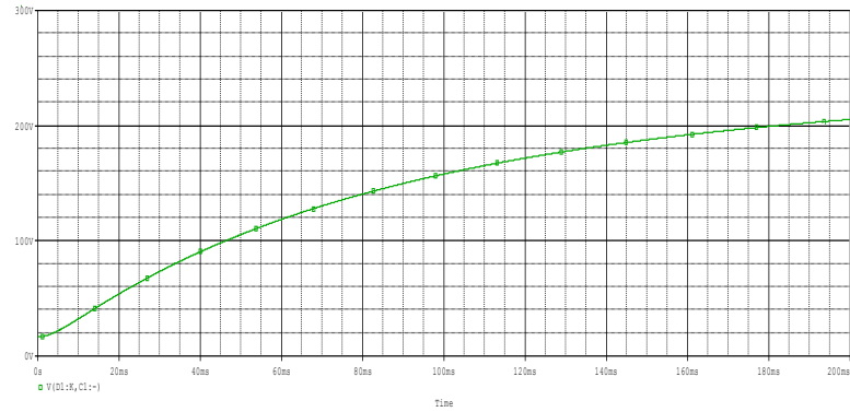
Fig. 9. It takes approximately 200 milliseconds to charge the capacitors to 200 volts in ideal conditions.
