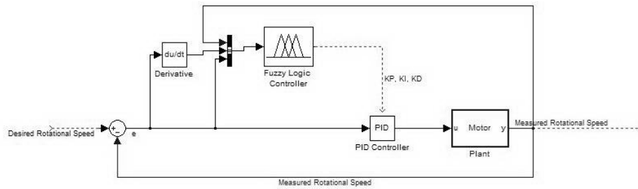
Fig.14. Low-Level Motor Controller Structure
