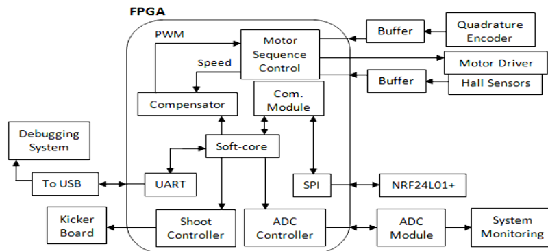
Fig. 6. Electrical system's Block Diagram
