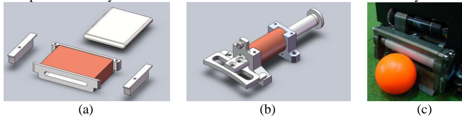
Fig. 4. (a) The new chip kick solenoid and plunger (b) The new linear kick solenoid and plunger (c) The dribbling system
