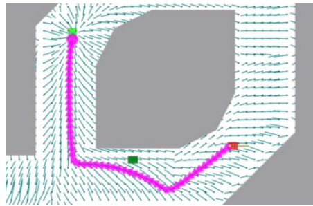
Fig. 7. The output plan of customized APF motion planner
