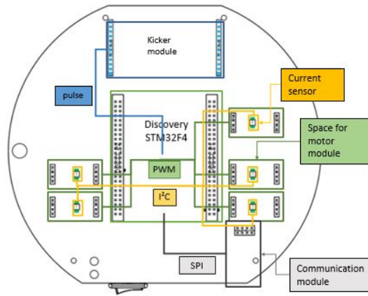
Fig. 5: Main board's block diagram
