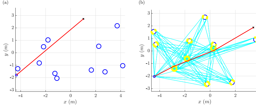
Fig. 15: Examples of plans computed by the A* circle-based visibility graphs: (a) direct visibility from source to goal, so no planning occurs (b) harder case where the robot has to evade obstacles to reach the goal.
