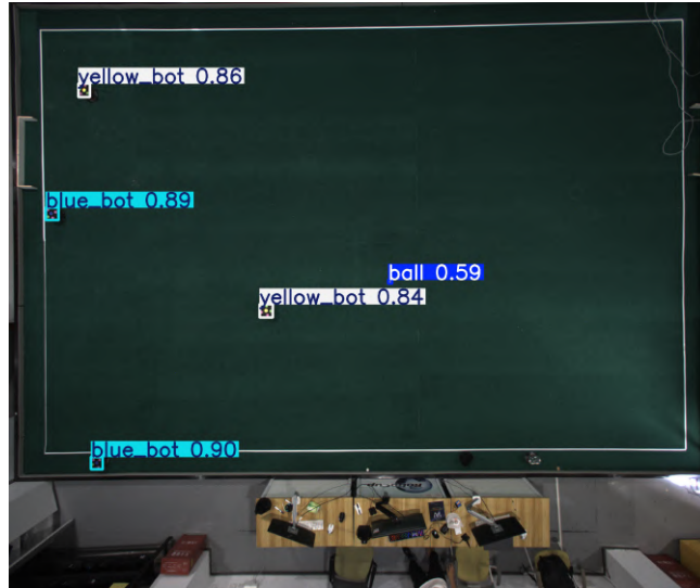
Fig. 4: The Detection Result of Yolov8 Model
