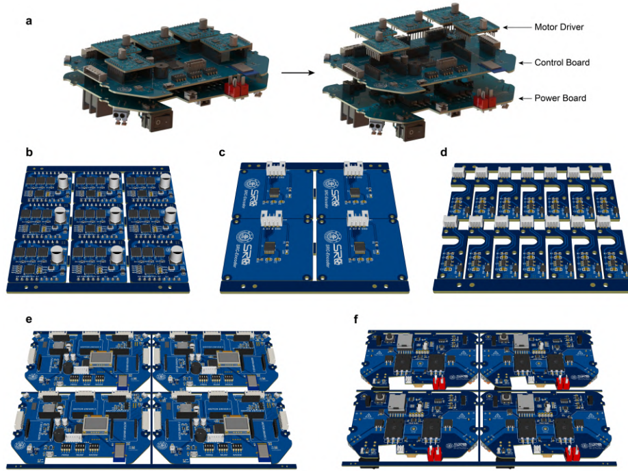
Fig.8: Electronic Control System Architecture of SRC 2026 Robot. (a)Assembly View of the Modular Design. And panelization design of the (b)motor driver, (c)encoder, (d)Infrared Sensor, (e)control board, (f)power board.
