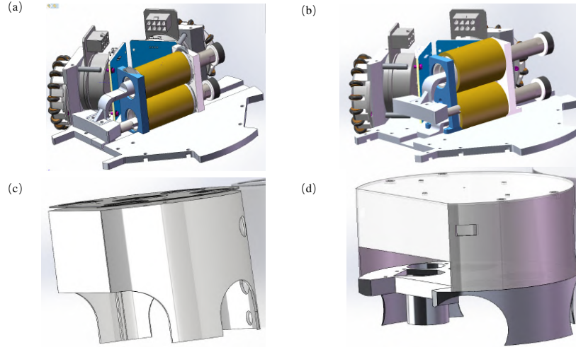
Fig. 10: SRC 2026 Kick Board & Shell. (a)(c)Before (b)(d)After
