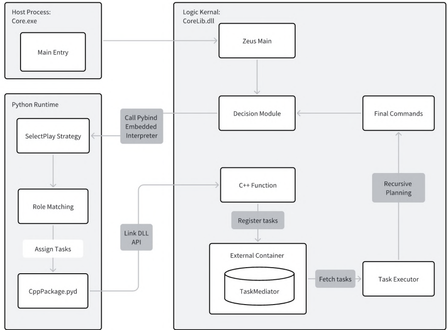
Fig. 2: Overview of Python-C++ Based Architecture.
