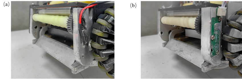
Fig. 11: SRC 2026 Infrared Sensor. (a)Before (b)After
