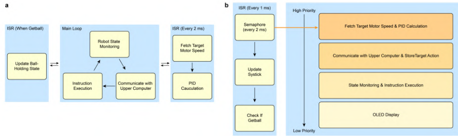
Fig. 7: Flowchart of SRC Embedded Firmware. (a) Simple embedded program. (b) Firmware based on FreeRTOS.
