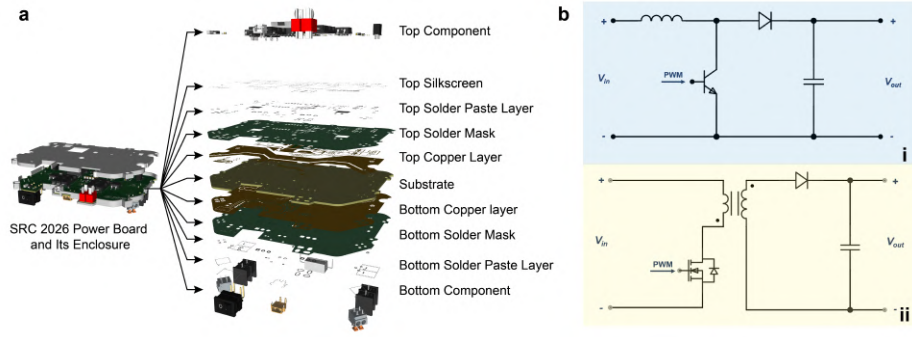
Fig. 6: SRC 2026 Power Board. (a)Power board and its laminated structure renderings. (b)Topological structures of (i)boost circuit and (ii)flyback circuit.
