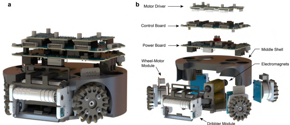
Fig. 1: SRC 2026 Robot. (a)Rendering image of the robot. (b)Explosion view of the robot.
