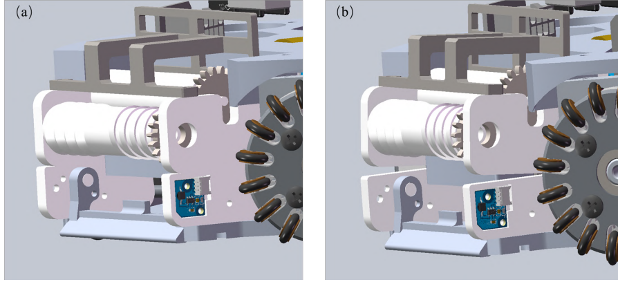
Fig. 9: SRC 2026 Dribbler. (a)Initial State, (b)Dribbling State
